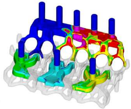
Casting Flow Analysis
