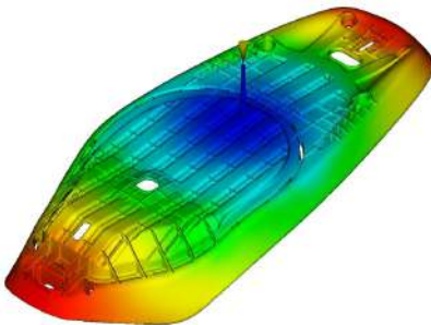
Mold Flow Analysis
