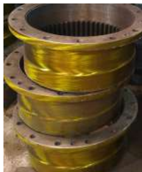
Geared Couplings
